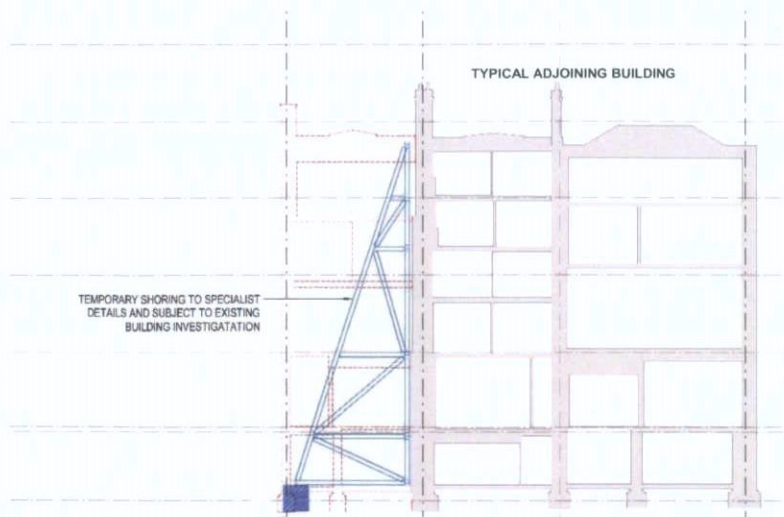
Figure 24 – Typical Temporary Boundary/Adjoining Retention System
