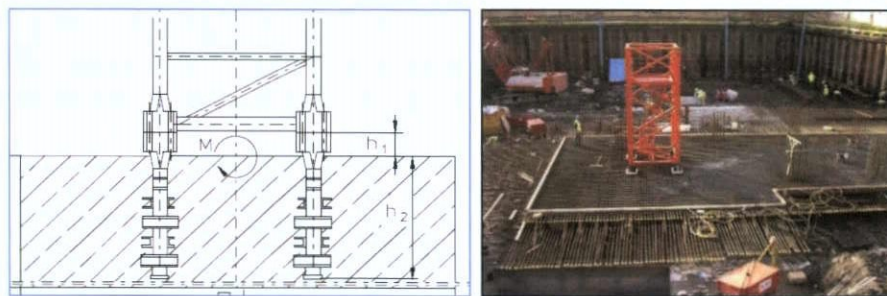
Figure 7 – Typical Tower Crane Anchors
