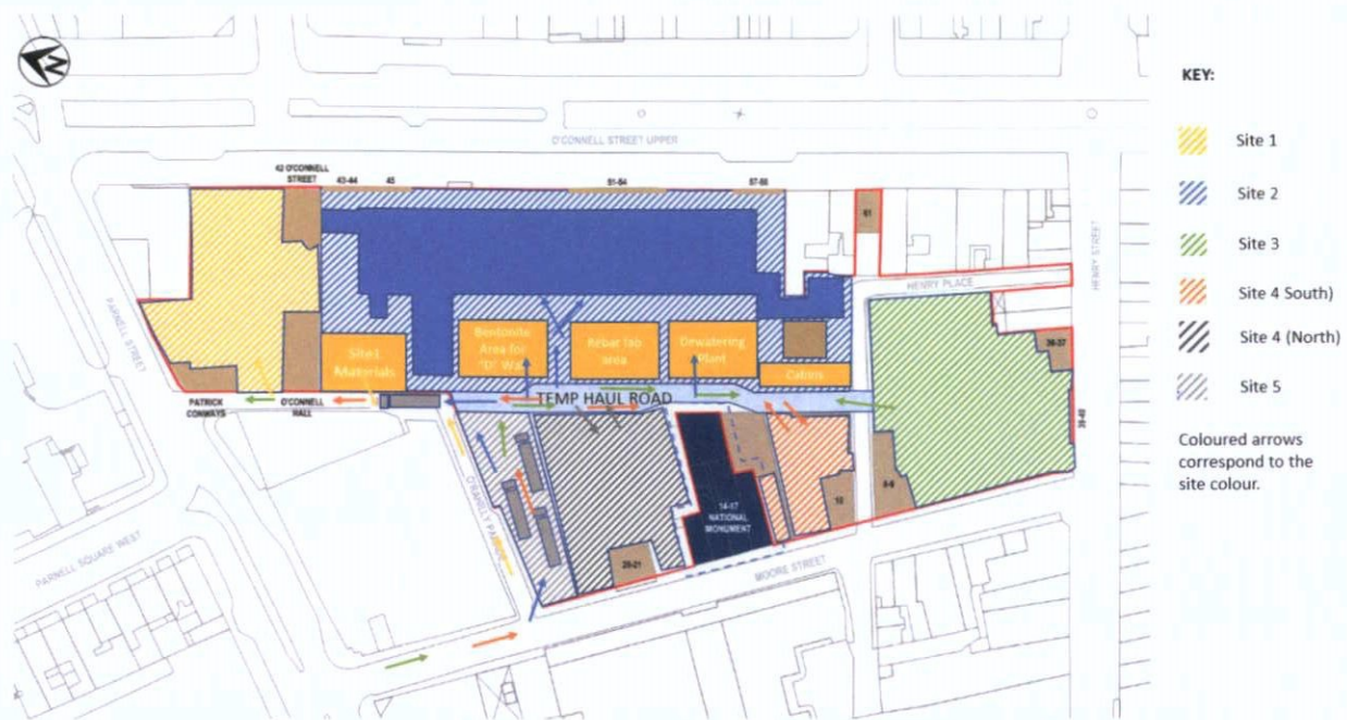
Figure 8 – Necessary site area for construction and access / egress points.
