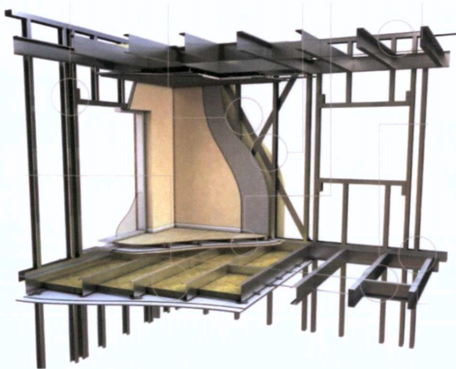
Figure 25 – Typical Metsec SFS System
